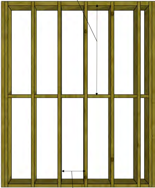
12" to 16" O.C.
